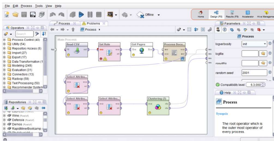
Figura 16 – RapidMiner Studio
