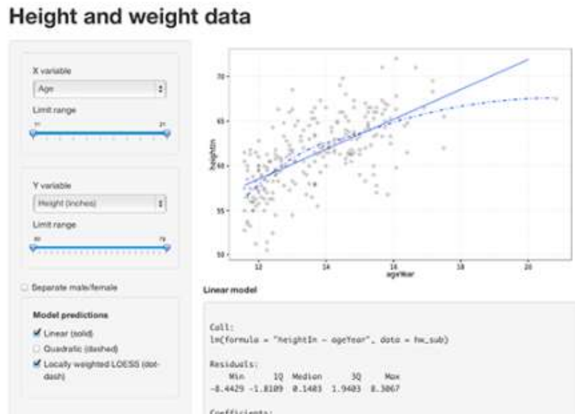
Figura 18 – Shiny
