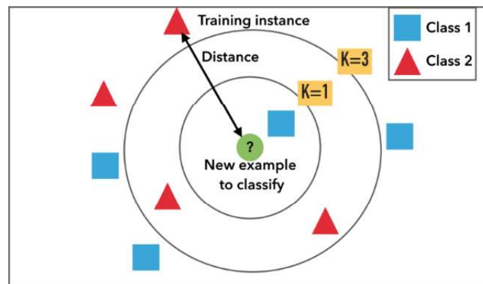
Figura 8 – k-Nearest-Neighbours
