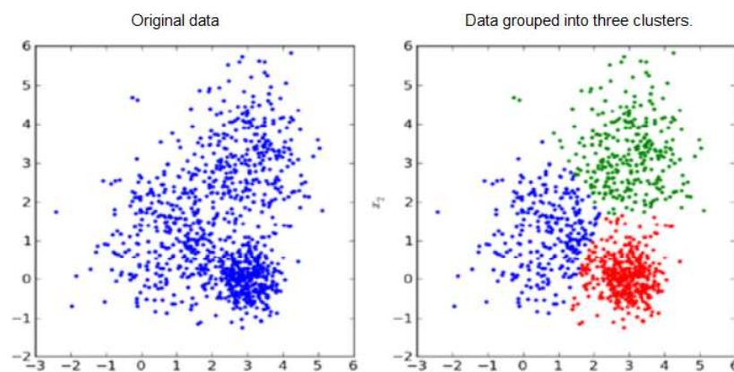
Figura 9 – K-Means Clustering
