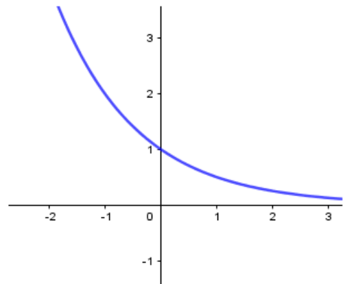
(b) 0 < a < 1
