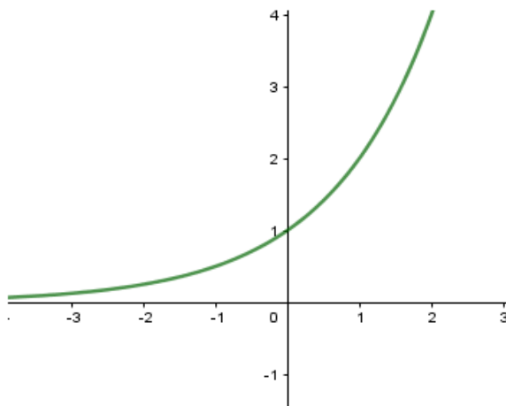
(a) a > 1
